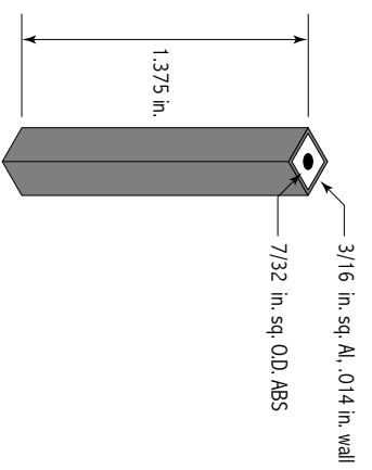
Standoff Detail
